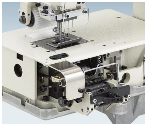
Mechanical elastic feeding device (option)
