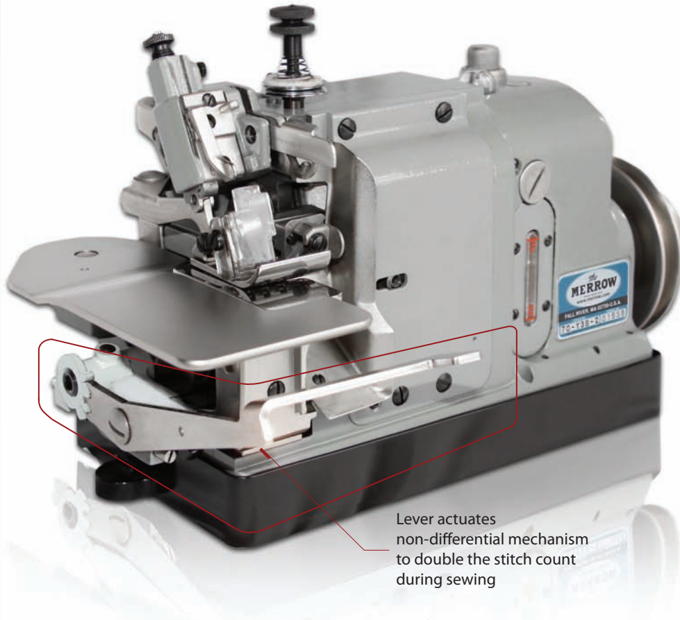
BUTTED SEAM
