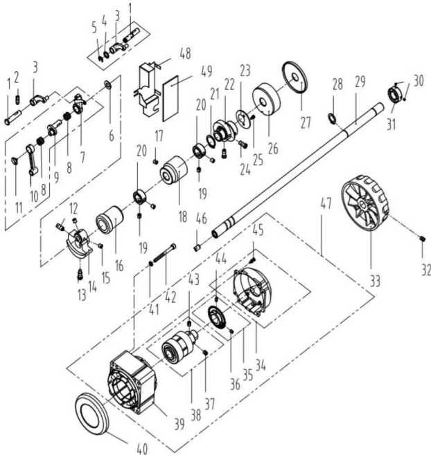
2. 上轴、挑线部件 /Main Shaft & Thread Take-up Components
