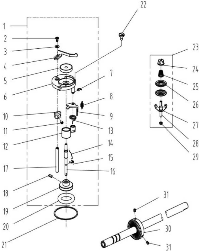
10. 绕线部件/ Winding Components
